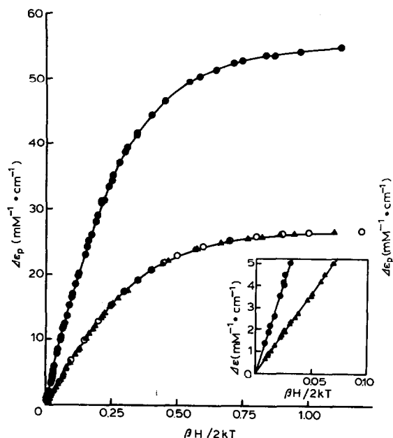
Fig. 8. MCD magnetization curves (i.e., plots of peak to trough intensity for the Soret-band MCD, \Delta\epsilon_p , versus \beta H/2kT ) for the oxidized resting ( \blacktriangle ) and oxidized cyanide ( \bullet ) derivatives of cytochrome c oxidase. The insert shows an expression of the region at low \beta H/2kT values. From ref. 46.
