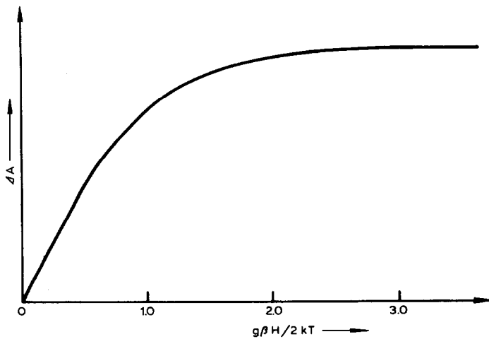
Fig. 2. MCD saturation curve for a system with a Kramer’s doublet ground state. From ref. 3.
