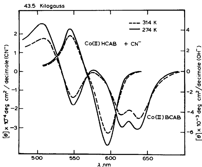
Fig. 14. MCD (at 4.35 T) of Co(II) bovine carbonic anhydrase B (BCAB) and Co(II) human carbonic anhydrase B · \text{CN}^- (HCAB + \text{CN}^- ) as a function of temperature; (—) 274 K; (---) 314 K. From ref. 66.
