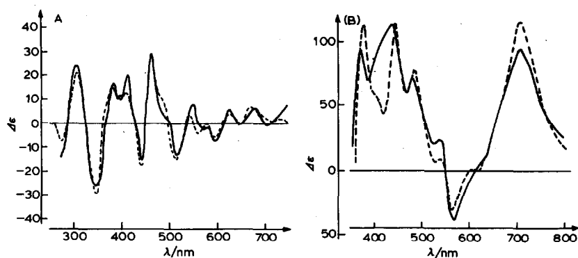
Fig. 23. (A) MCD spectra of ferricyanide-oxidized Clostridium pasteurianum ferredoxin (—) and oxidized ferredoxin II from Desulfovibrio gigas (-----) at 4.215 K and 5.13 T. The \Delta\epsilon scale refers only to the spectrum of ferredoxin II. The spectra have been normalized at 462 nm. From ref. 142. (B) MCD spectra of dithionite-reduced, ferricyanide-oxidized Clostridium pasteurianum ferredoxin (—) and dithionite-reduced ferredoxin II from Desulfovibrio gigas at 4.215 K and 5.13 T. The \Delta\epsilon scale refers only to the spectrum of ferredoxin II. The spectra have been normalized at 500 nm. From ref. 142.
