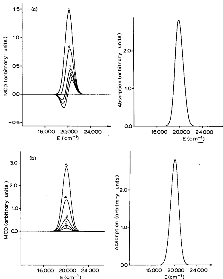
Fig. 1. Magnetic circular dichroism dispersion according to the rigid shift model. In (a) the effect of varying the relative magnitudes of the A and (B + C) terms is illustrated. The zero-field absorption is calculated for a bandsshape function, f = \Delta^{-1} \pi^{-1} \exp[-(E - E^0)^2/\Delta^2] , E^0 = 20000 \text{ cm}^{-1} , \Delta = 1000 \text{ cm}^{-1} . The MCD is calculated from eqn. (1) with A_1 = 1 , \beta H = 1 \text{ cm}^{-1} and (B_0 + C_0/kT) equal to: (1) 0; (2) 5 \times 10^{-4} ; (3) 1 \times 10^{-3} ; (4) 2.5 \times 10^{-3} ; (5) 5 \times 10^{-3} . In (b) the effect of varying the temperature ( T ) on the C terms is illustrated. The zero-field absorption is identical to (a). The MCD is calculated with A_1 = B_0 = 0 , C_0 = 1 and kT equal to: (1) 200 \text{ cm}^{-1} ; (2) 100 \text{ cm}^{-1} ; (3) 50 \text{ cm}^{-1} ; (4) 20 \text{ cm}^{-1} ; (5) 10 \text{ cm}^{-1} . Adapted from ref. 3.
