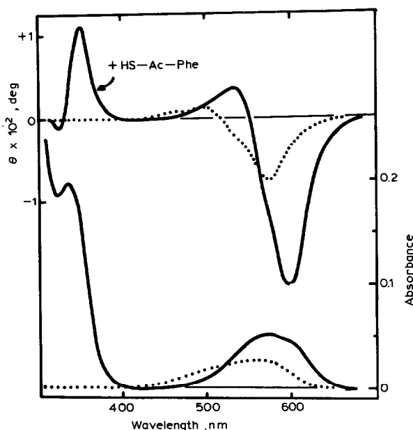
Fig. 19. Absorption (lower) and MCD spectra (at a magnetic field of 4 T) of Co(II) substituted carboxypeptidase A ( 2.8 \times 10^{-4} M) in the absence (·····) and presence (—) of the inhibitor 2-mercaptoacetyl-D-phenylalanine (HS-Ac-Phe). Adapted from ref. 97.
